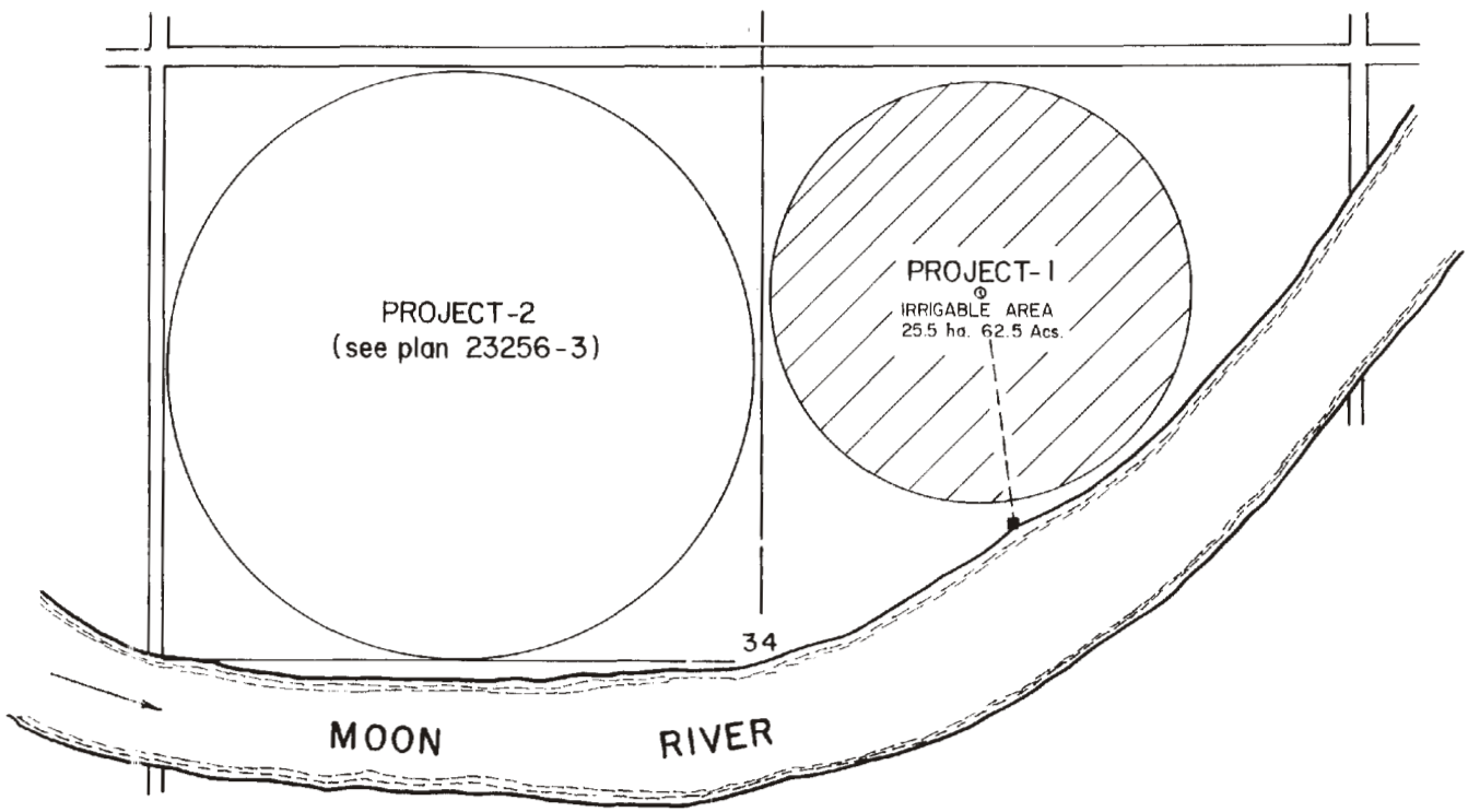
GENERAL PLAN
